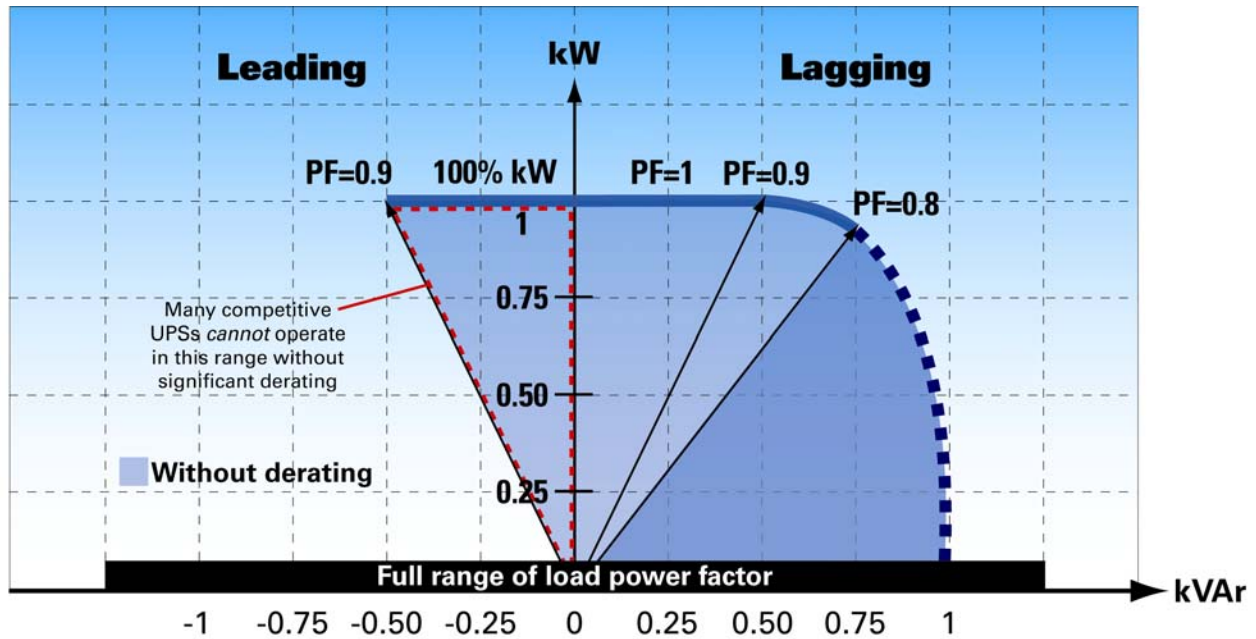
Figure 1: Full Range of Load Power Factor for Powerware® UPS
